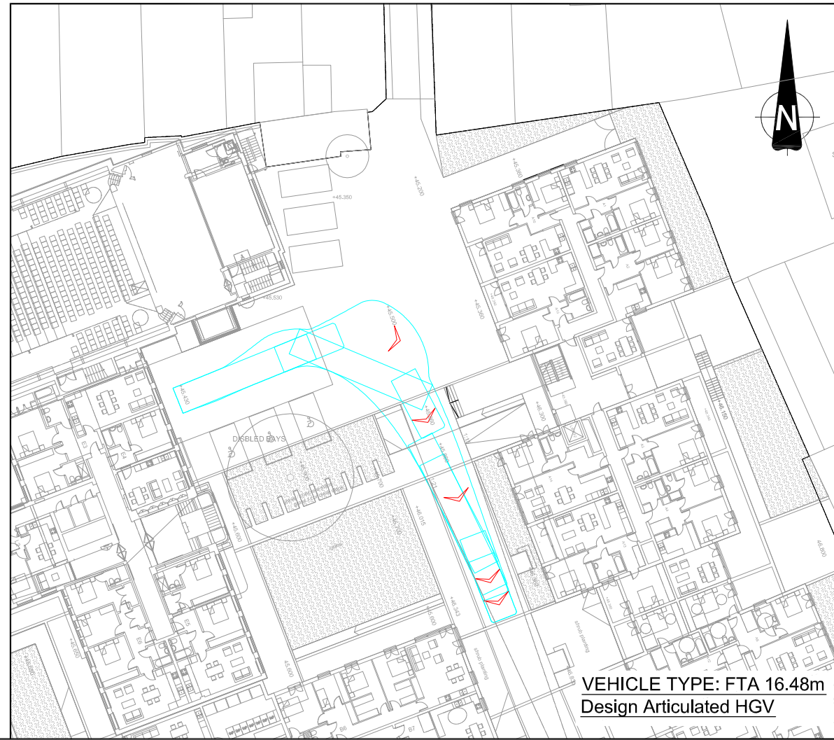
VEHICLE TYPE: FTA Design 10.0m Ridgid HGV
